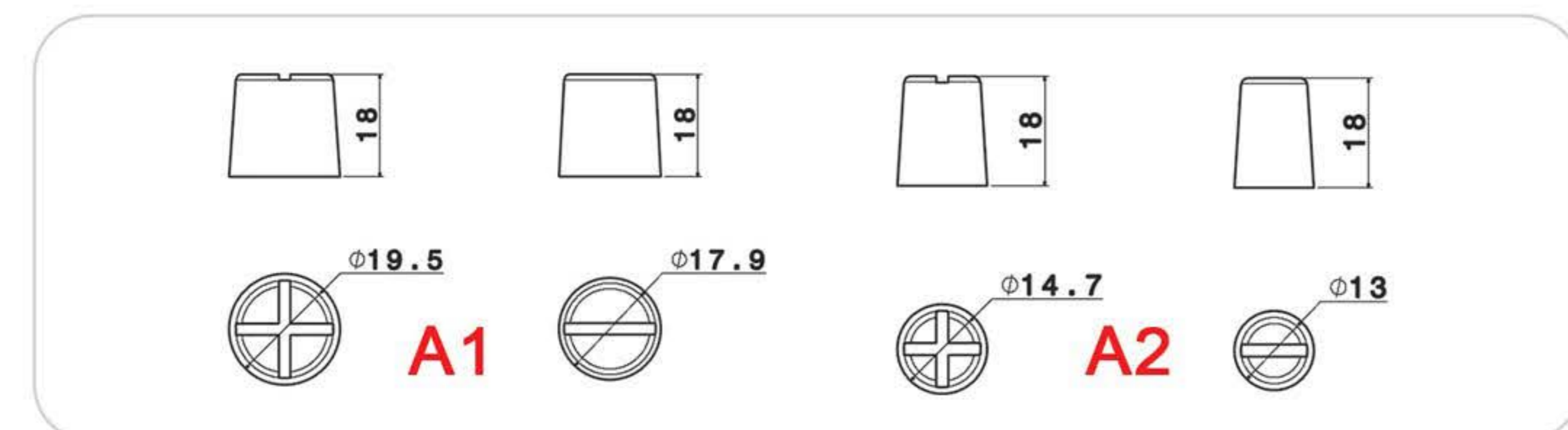
Battery Terminals
